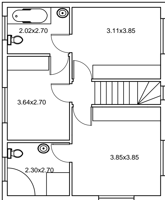
A First Floor Plan Scale 1:100
