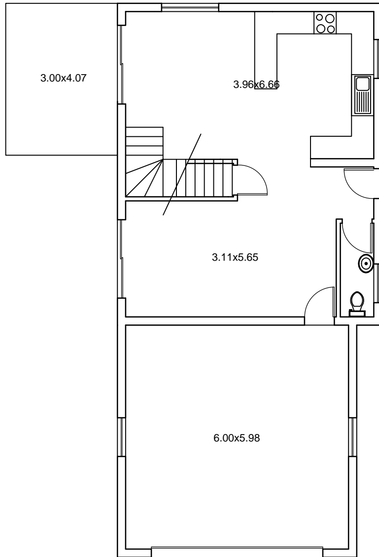
B Ground Floor Plan Scale 1:100 Area: 113sq/m
